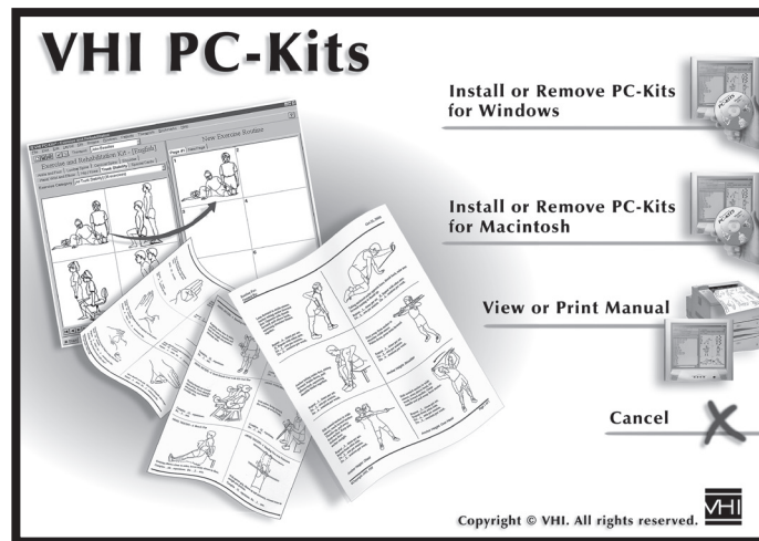
Figure 1. Splash Screen
